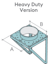
Heavy Duty Version Model 2 650mm - 1200mm B= Fixing Hole Centres Installed height of Support Length 170mm. Corresponding Cover Jacket set required (See Page 21)
