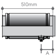
25mm Cavity
